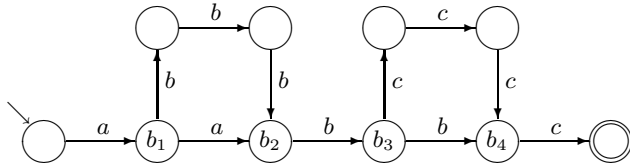
Fig. 5. The minimal N-DFA \mathcal{A} for L = \{a^2b^2c, a^2bc^4, ab^5c, ab^4c^4\}
