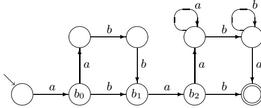
Fig. 4. The minimal N-DFA \mathcal{A} for L = \{aabbbaa^+b^+a, abaa^+b^+a, aabbab, abab\}
