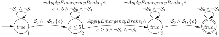
Fig. 3. Test automaton for [true] \Downarrow_{S_0} \text{NoBrake}_1 \Downarrow_{S_1} [true]
