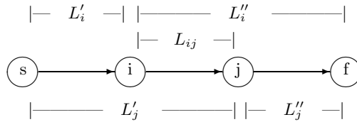
Fig. 2. Decompositions of L(\mathcal{A}) corresponding to the strong bridge states i and j
