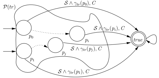
Fig. 2. Sequential composition (illustration)
