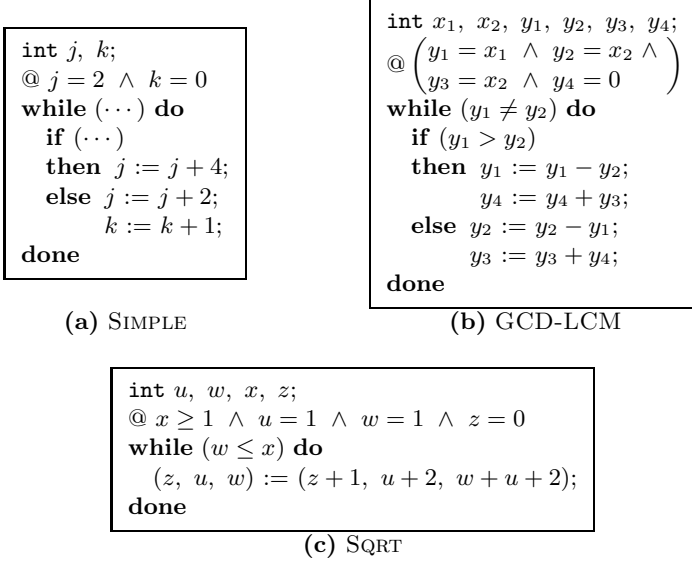
Fig. 1. Example functions
