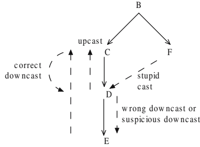
Fig. 1. The Inheritance Tree for Classes
